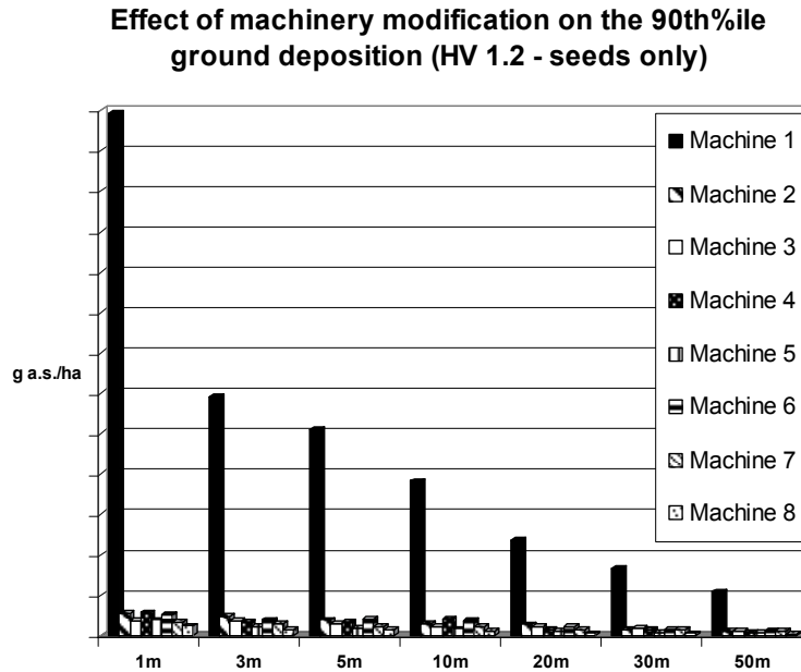
Figure 11 Effect of machinery modification on off-crop ground deposition. Machine 1 is an unmodified reference machine, machines 2-8 are all low-drift machinery
