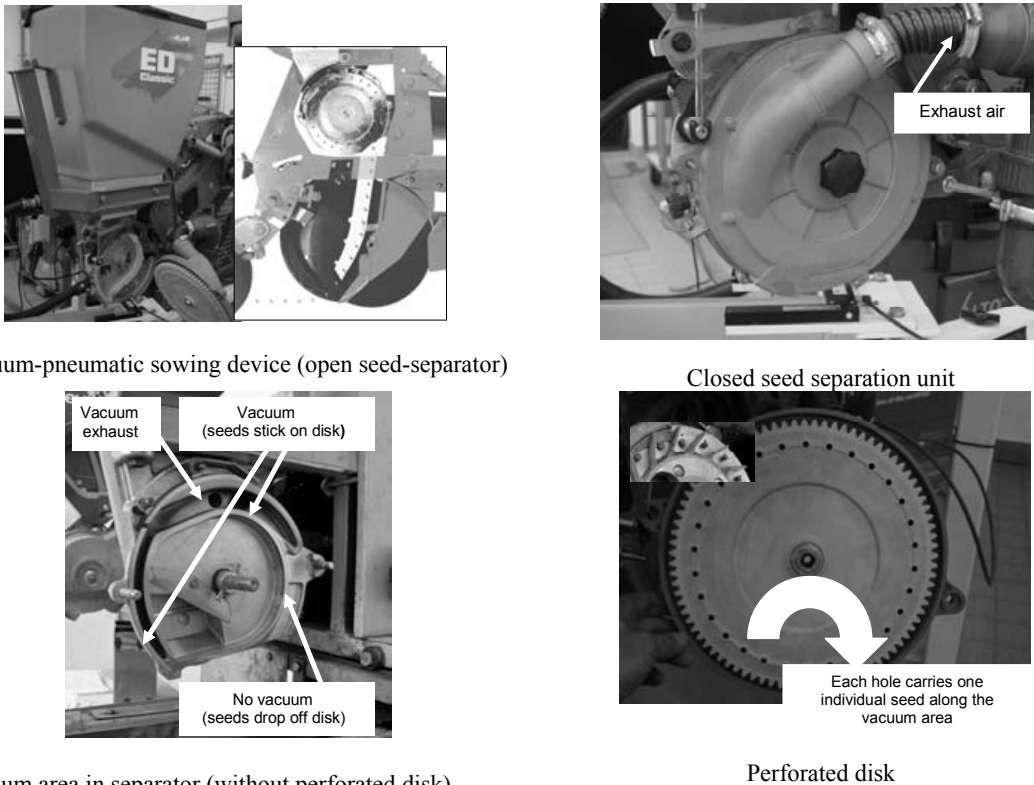
Vacuum area in separator (without perforated disk)
